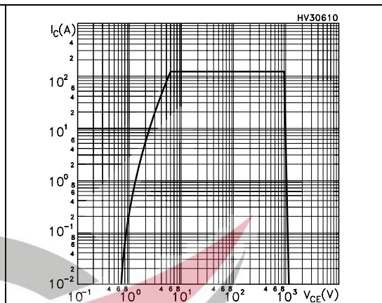
Figure 15. Turn-off SOA
